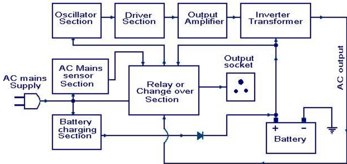
Block diagram of a basic inverter
