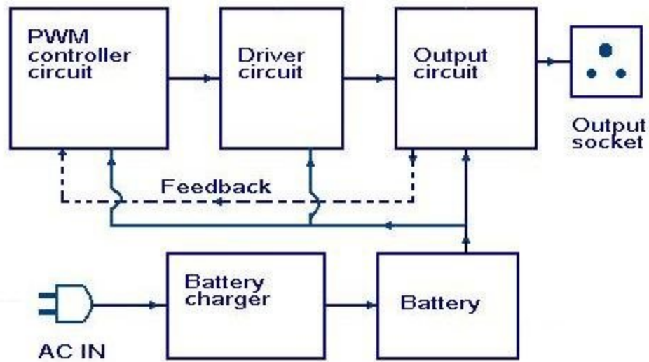
Block diagram of a basic PWM inverter
